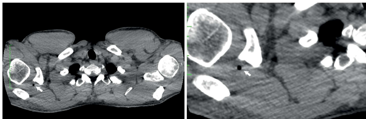
Residual tissue bubbles after recompression
